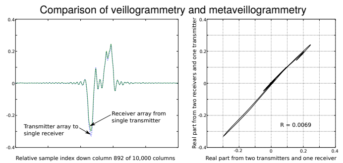
Fig. 14. Comparison between double transmit and single receive (veillogrammetry) and double receive and single transmit (metaveillogrammetry).
