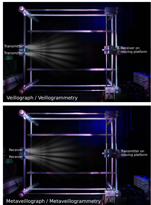
Fig. 13. Top: photograph of a sound wave emanating from two speakers. Bottom: photograph of a veilance wave function "emanating" from two microphones (i.e. a photograph of the capability of two microphones to "hear").
