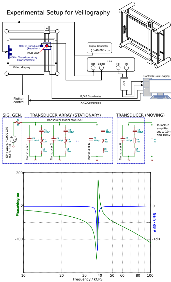
Fig. 12. Apparatus (with equivalent circuit schematic and frequency response) for the experimental comparison between veillography and metaveillography. Here is shown the apparatus connected for veillography, with a stationary array of transmitters (speakers) and a moving receiver (microphone). This corresponds to the top picture in Fig. 12. For metaveillography (bottom picture of Fig. 12), the connections between the stationary transducer array and the moving transducer are simply swapped.
