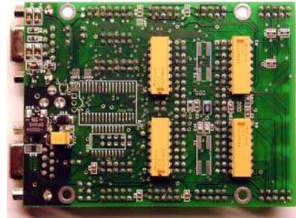
Figure 3: AVRmini (bottom)
