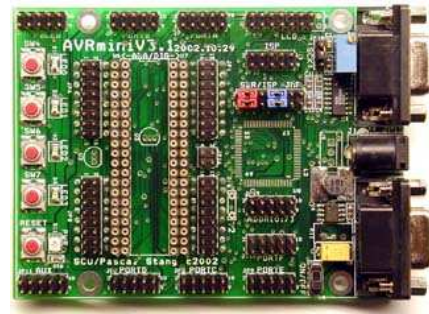
Figure 2: The AVRmini Development Board (top)
