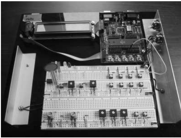
Figure 1: Prototyping Kit
